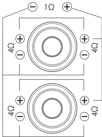
PARALLEL / PARALLEL
