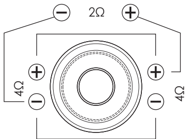
PARALLEL
