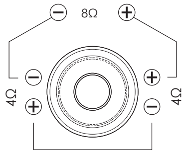
SERIES
