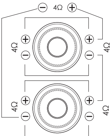
PARALLEL / SERIES
