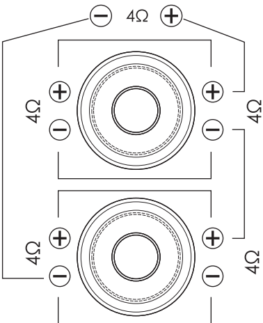
PARALLEL / SERIES
